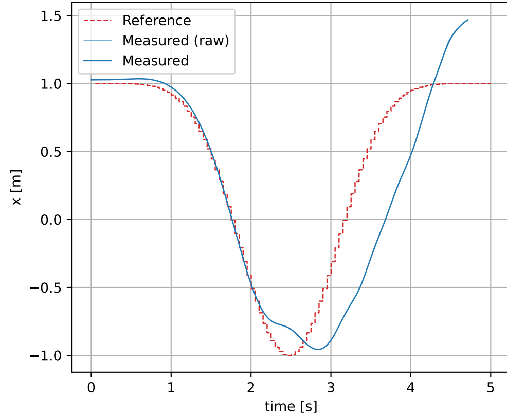
x State
