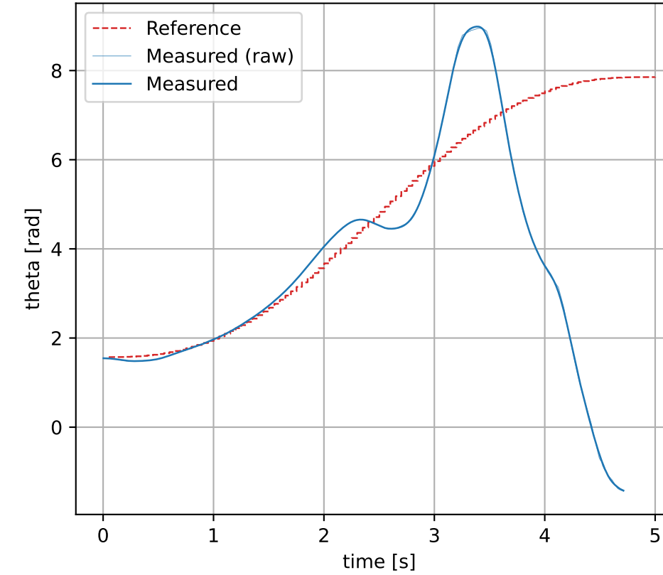
theta State
